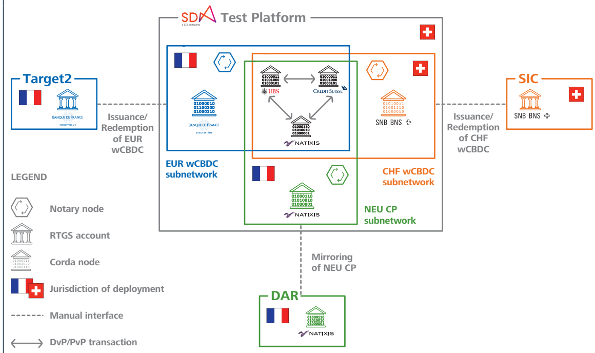
FIGURE 2 – Experimental architecture
